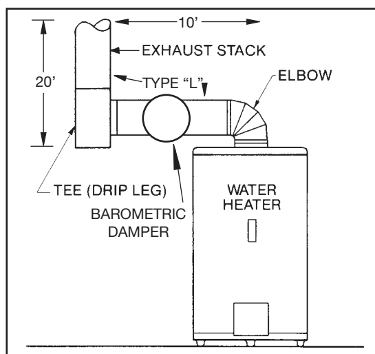
Figure 22: Typical Individual Venting
